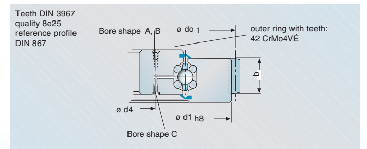
Outer gear
