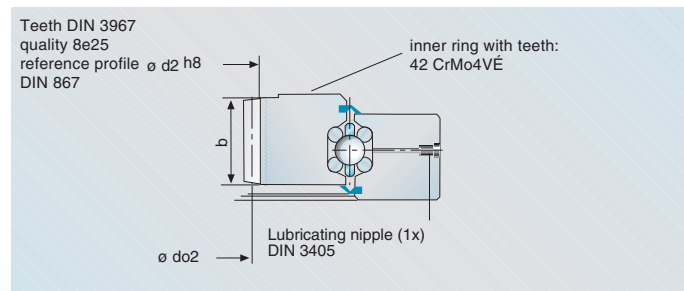
Inner gear
